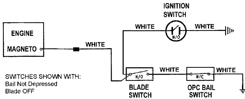
Wiring Schematic for GM2513H (Honda) model with Harness # 1723632
