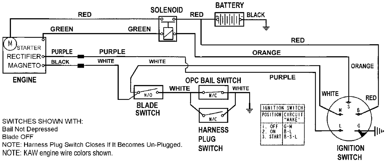
Wiring Schematic for GM2513BS (Briggs) model with Harness # 7044922 and for GM2515KAW (Kawasaki) model with Harness # 7044926
